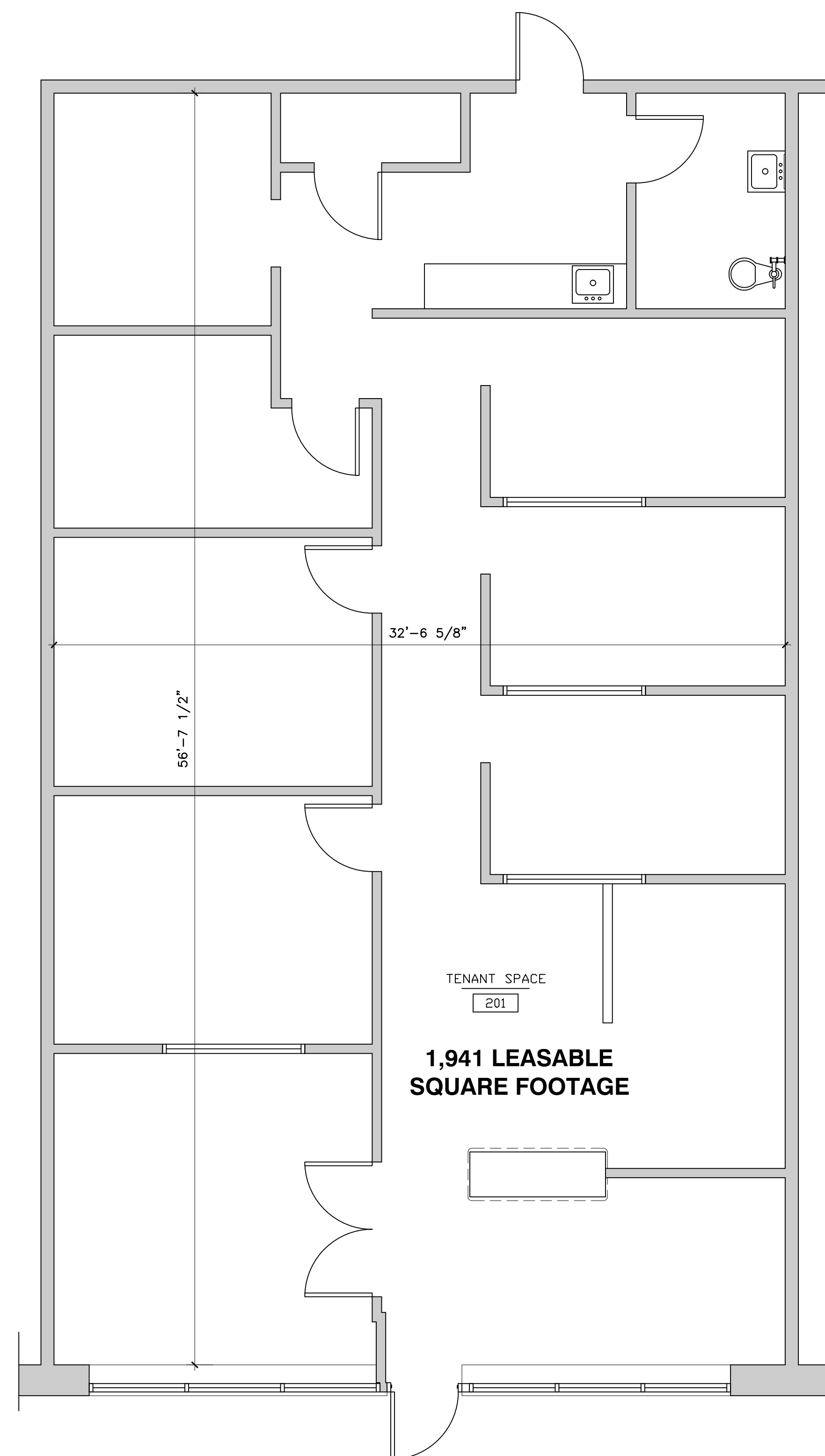
1 TENANT LEASE PLAN SCALE: 1/4" = 1'-0"
